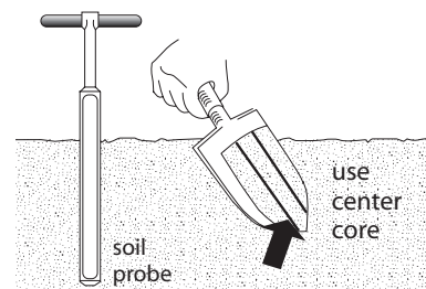
FIGURE 1. Sampling tools
